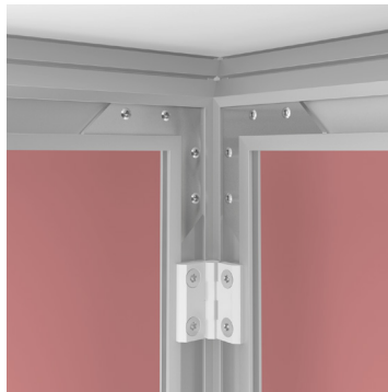
OCTACOUNTER FABRIC DETAIL TÜRBAND
